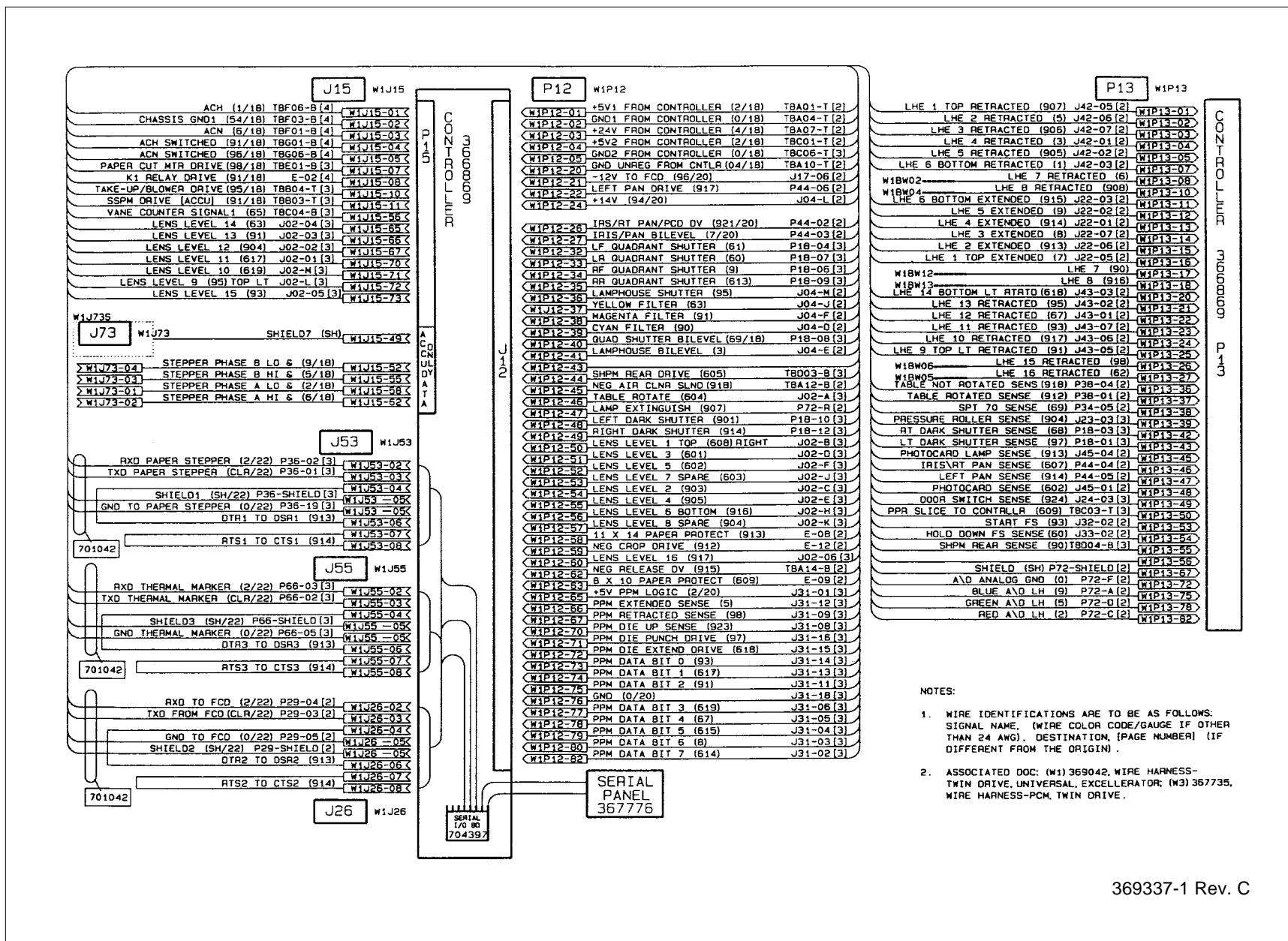
Figure 15 — Twin Drive Machine Schematic 1 of 5
