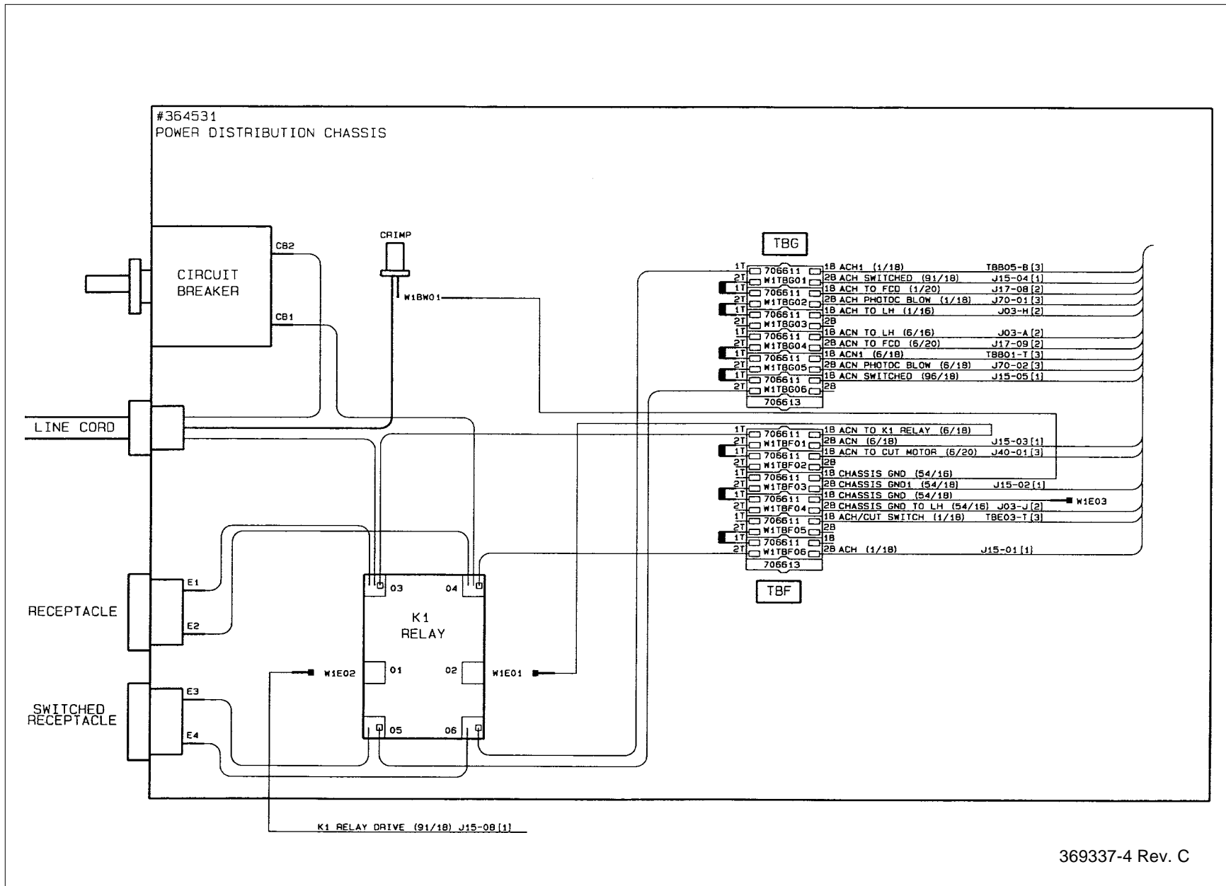
Figure 18 — Twin Drive Machine Schematic 4 of 5
