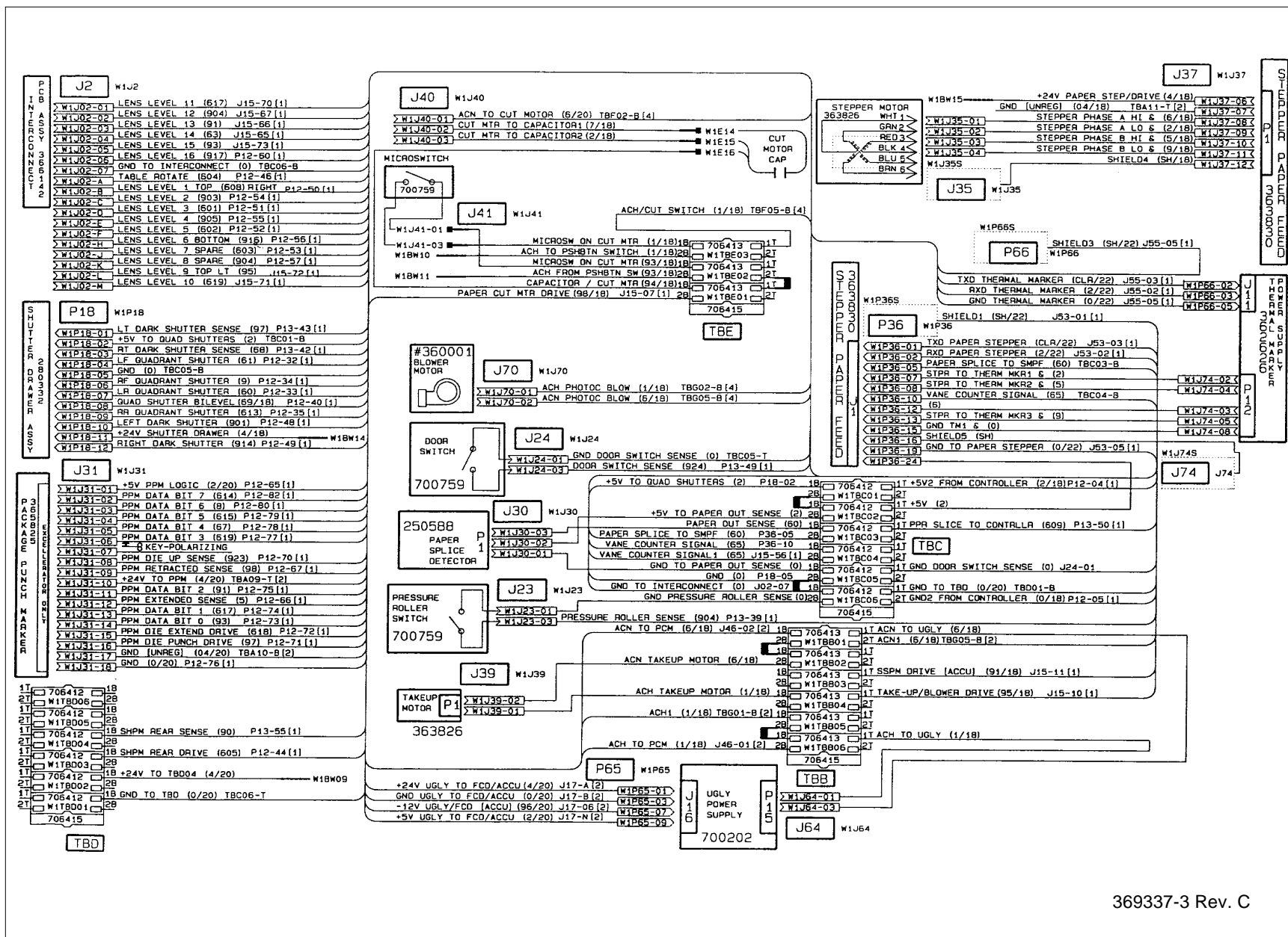
Figure 17 — Twin Drive Machine Schematic 3 of 5
