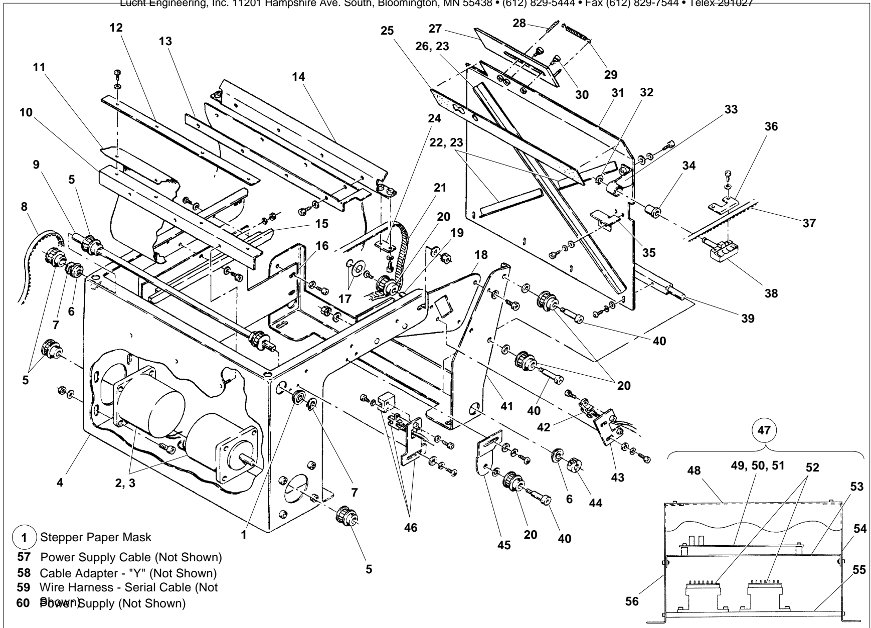
Figure 4 — Stepper Paper Mask
