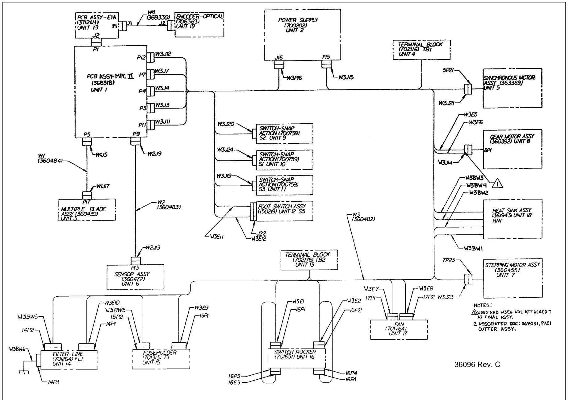
Wiring Diagram - PPC
